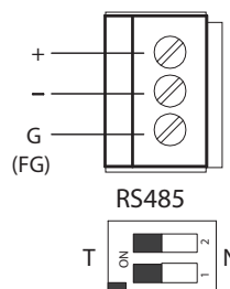
Pin assignment of the connector
