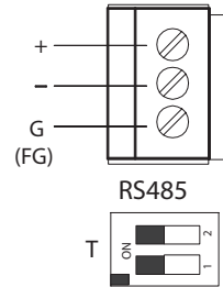
Pin assignment of the connector
