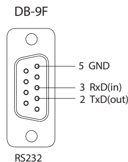
Pin assignment of the connector
