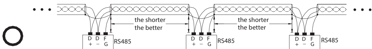
BUS connection
