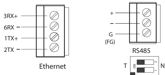
Pin assignment of the connector
