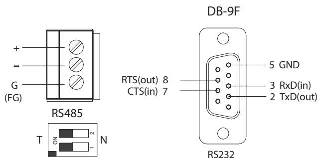
Pin assignment of the connector
