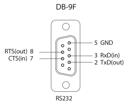
Pin assignment of the connector
